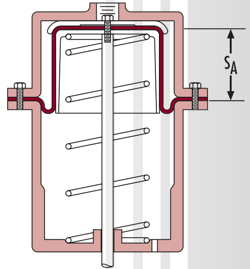
Fig. 7: Up-Stroke Position
