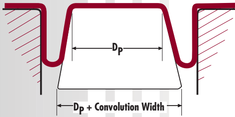
Fig. 40: Tapering the Piston
