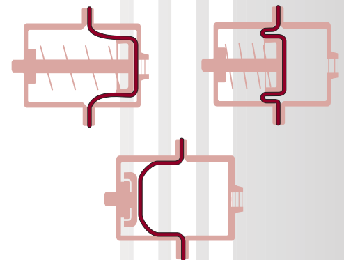
Fig. 13: Involved Diaphragm cycle. Convolution is not required at stroke limits.
