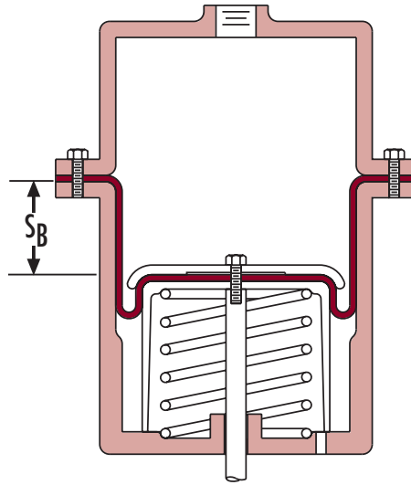
Fig. 6: Down-Stroke Position
