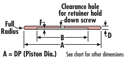
Fig. 19: Flat washer type retainer for Classes 3C and 4C (Pre-convoluted Diaphragms).
